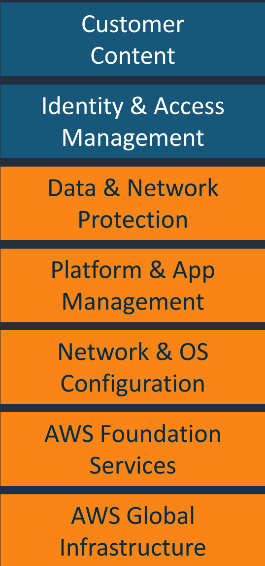
Serverless
