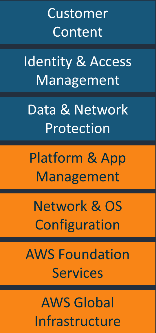
Managed Utility
